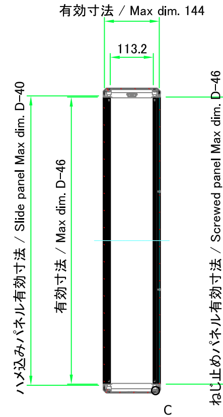
B-B (1:10)
